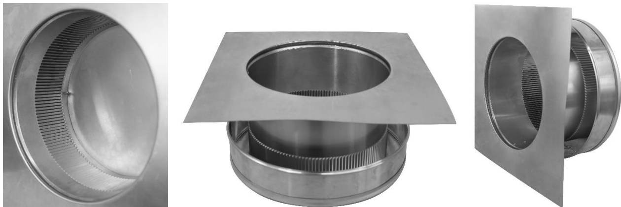
Figures 1-4: Side View, Angled Top View, Inside & Outside View of Louvers
